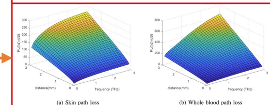
Fig. 3: Skin and whole blood path loss as function of distance and frequency.
